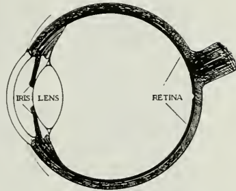
Fig. 6. Diagram of Human Eye.
